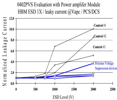
Figure 6: GaAs leakage degradation increases significantly at lower ESD voltages without PVS protection
