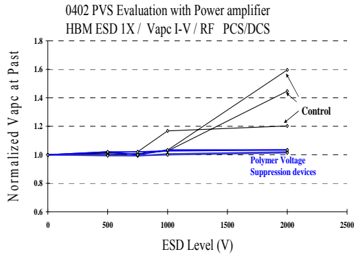
Figure 5: Device power setting degradation takes place at significantly lower ESD voltages without PVS protection.
