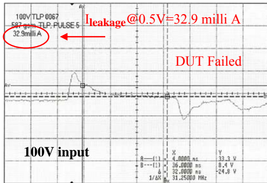
Figure 9: 100V VFTLP pulse into GaAs module increase damage to module
