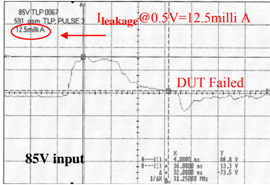
Figure 8: 85V VFTLP pulse in GaAs module damaged module
