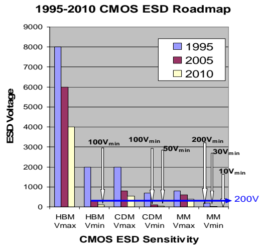
Figure 1: The National ESDA Technology Road Map shows engineers are sacrificing ESD reliability for performance
