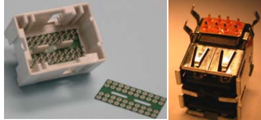
Figure 3: EPI-FLO™ ESD Connector Array on 40 pin MQS automotive ECM connector and a USB.
