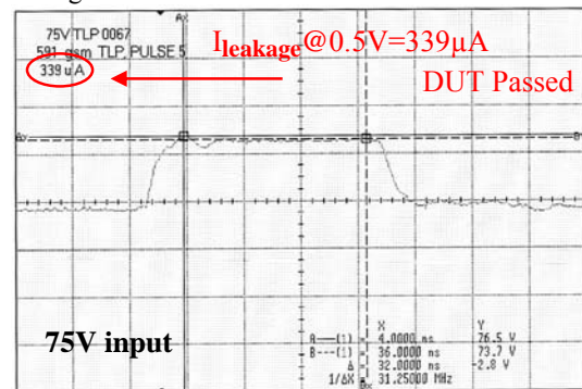
Figure 7: Scope trace for 75V VFTLP pulse into GaAs module shows no damage to the device
