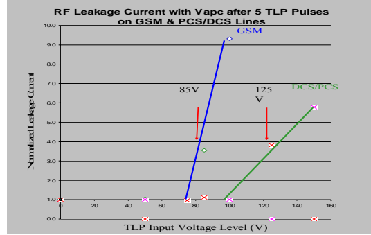
Figure 10: VFTLP damage threshold degradation curves from leakage current measurements at 1.5V
