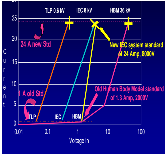
Figure 2: TLP testers and test protocols bridge the gap between system and semiconductor ESD standards
