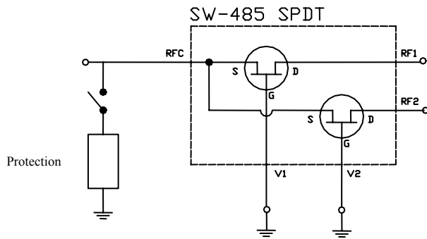
Figure7: Test setup for ESD and TLP testing of RF switch.
