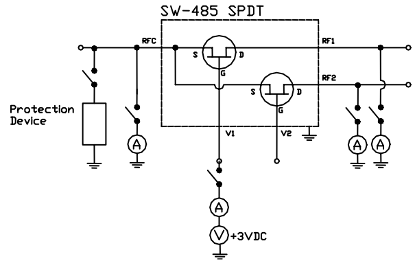
Figure 8: Generic post ESD/TLP test verification of device damage setup.
