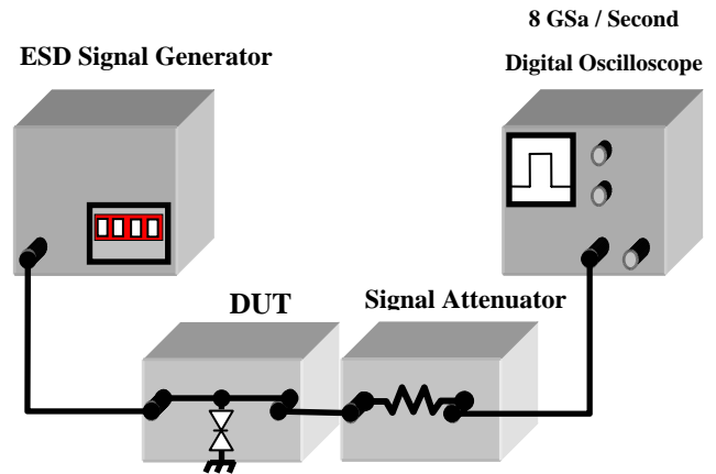
Figure 5: TLP set-up
