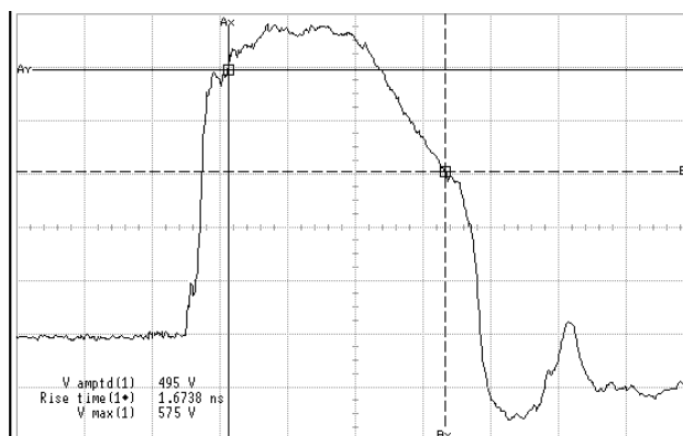
Figure 10: 600V TLP pulse input to RJ-45 connector with magnetics on PCB in the connector
