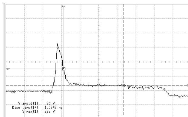
Figure 11: 600 V TLP into PVS protected RJ-45 Connector with magnetics on PCB in the connector
