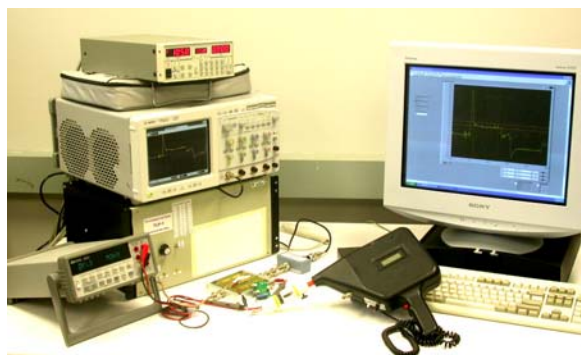
Figure 6: ESD Gun and TLP used for system level tests of components
