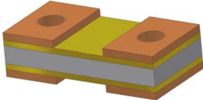
Figure 1: PVS Construction for 0603, 0402, 0201 Surface Mount Device
