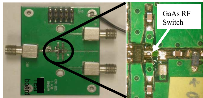
Figure 9: RF switch setup for ESD and TLP testing
