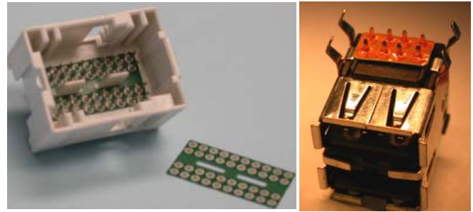
Figure 2: ESD Connector Array on 40 pin MQS automotive engine control module connector and 8 pin USB connector.
