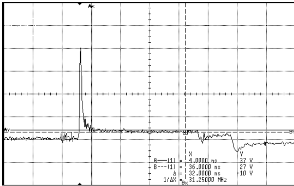
Figure 3: 0603 PVS device clamps 600 V TLP to 27 V
