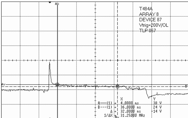
Figure 4: 200 V trigger 0603 PVS response to 200 V TLP.
